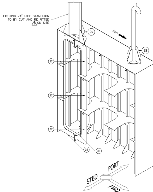
PERSPECTIVE VIEW WITHOUT SHELL PLATE SCALE: N.T.S.
