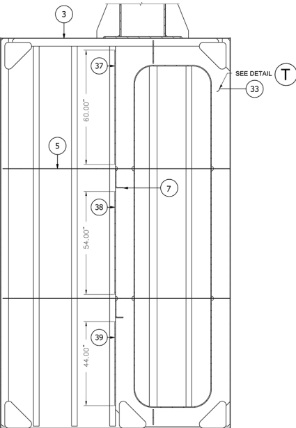
SECTION S LOOKING AFT SCALE: 1/2"= 1'-0"
