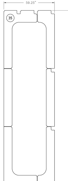
DETAIL U STANCHION SUPPORT NOTE - OVER ALL DIMENSIONS ONLY PARTS TO BE WATER CUT SCALE: 1/2"= 1'-0"
