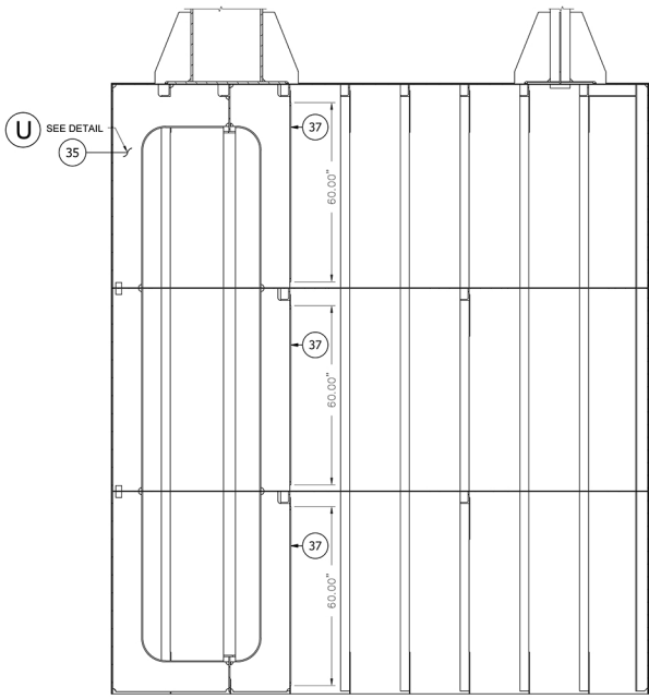
SECTION R LOOKING TO PORT SCALE: 1/2"= 1'-0"
