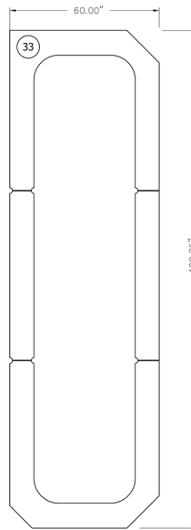
DETAIL T STANCHION SUPPORT NOTE - OVER ALL DIMENSIONS ONLY PARTS TO BE WATER CUT SCALE: 1/2"= 1'-0"
