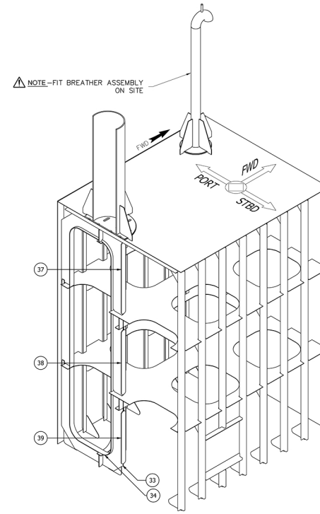
PERSPECTIVE VIEW WITHOUT SHELL PLATE SCALE: N.T.S.
